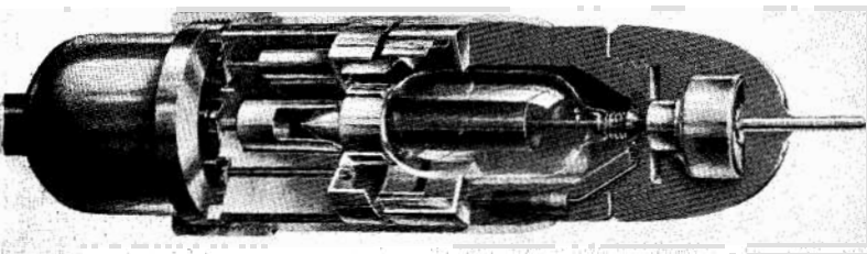
Figure 1. Construction details of new -hp- diode probe
