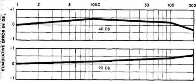
Figure 1. Typical Frequency Response
